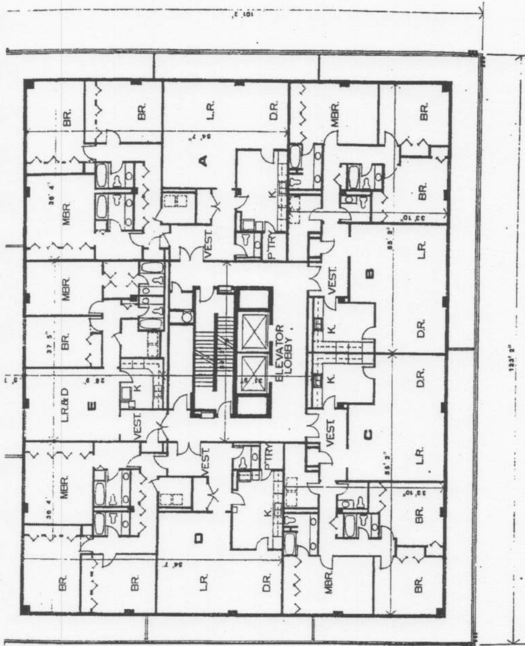
FLOOR PLAN 10, 11, 16, 17TH FLOORS 4 THREE BEDROOM & 1 TWO BEDROOM UNITS
